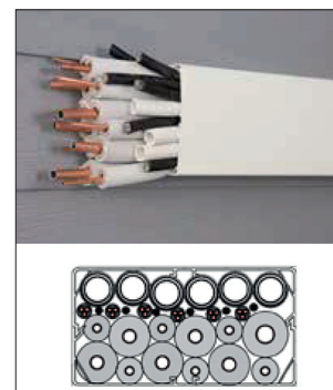
150 X 80MM
